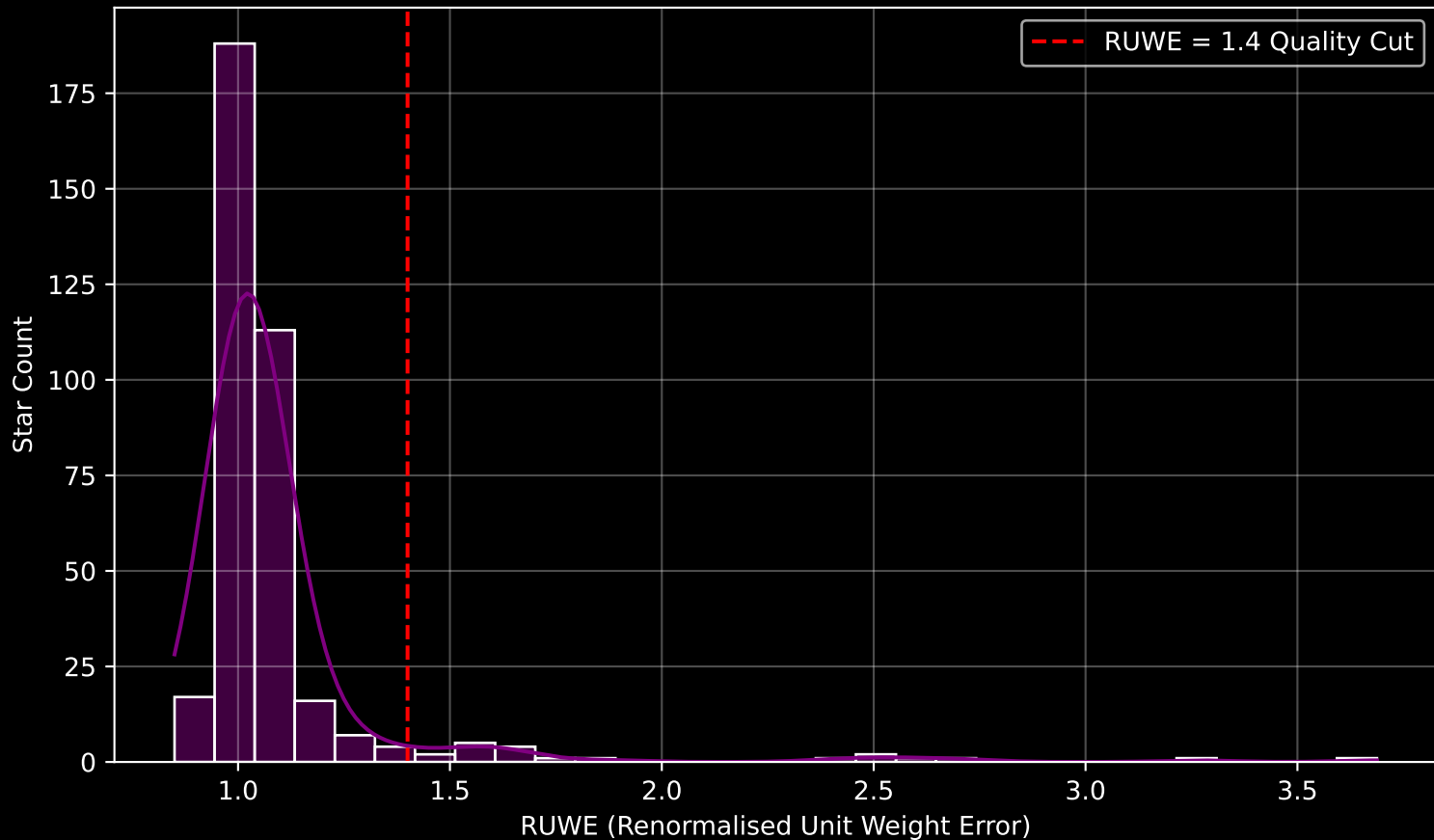
GAPOGEE DR17 Field [169-08] RUWE Distribution (n= 365)
