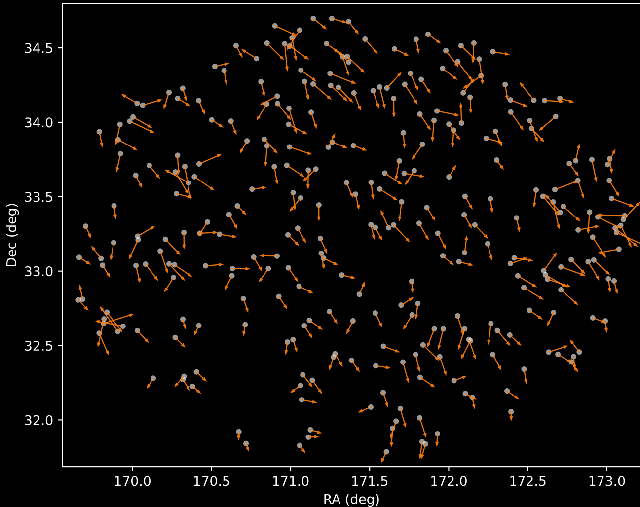
APOGEE DR17 Cluster 2 Proper Motion Vectors (n=295)
