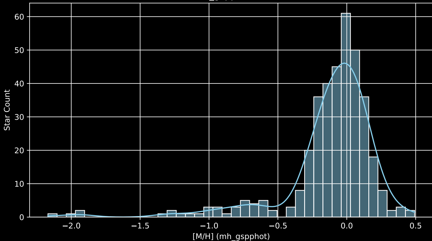
APOGEE DR17 Field: [169-08 [M/H] (mh_gspphot) (n= 368)
