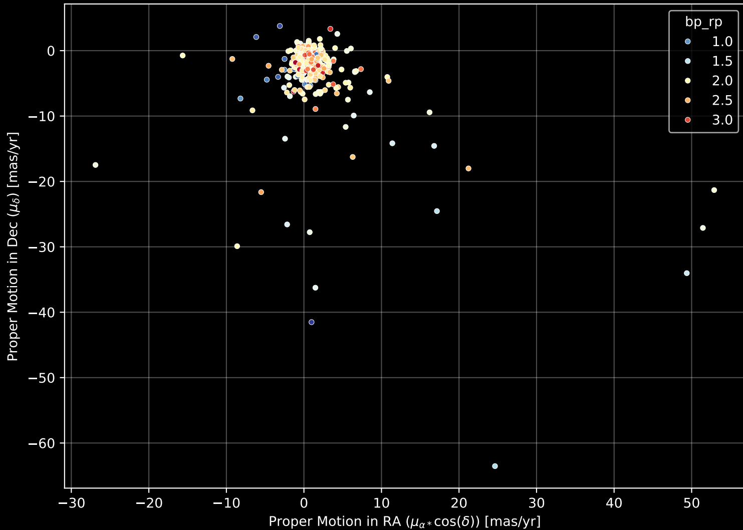
APOGEE DR17 Field: [169-08] Proper Motion Diagram (n= 369)
