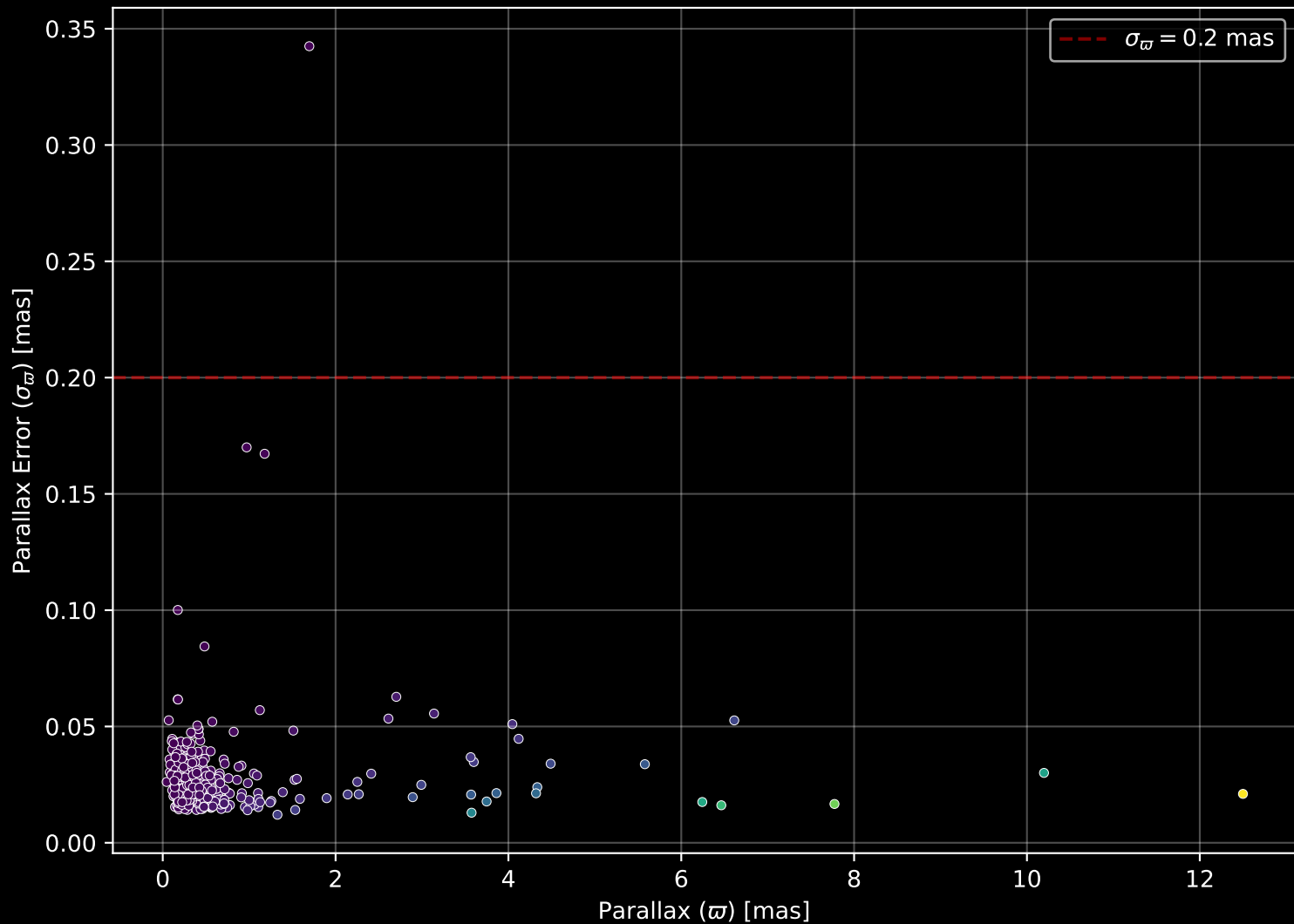
APOGEE DR17 Field: [169-08] Parallax Quality (n= 369)
